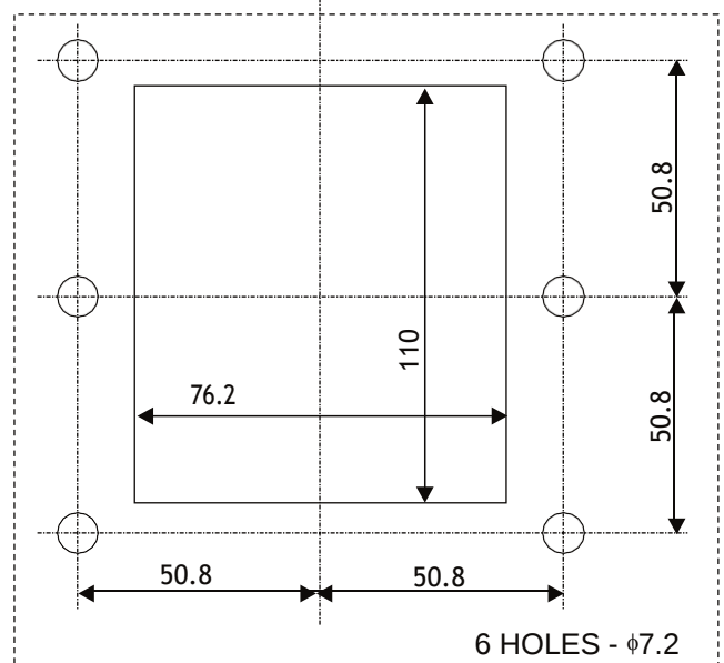
Details for side mounting
